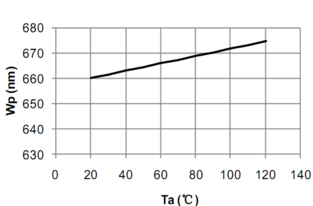
Peak Wavelength (@350mA) vs. Ambient Temperature
