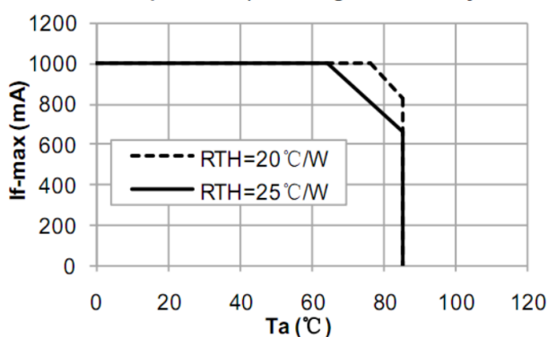
Maximum Driving Forward DC Current vs. Ambient Temperature (Derating based on Tjmax=125°C)
