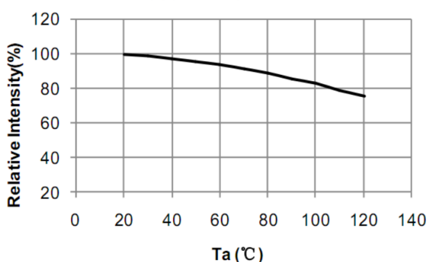
Relative Intensity(@350mA) vs. Ambient Temperature
