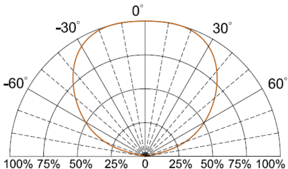
Directivity Radiation
