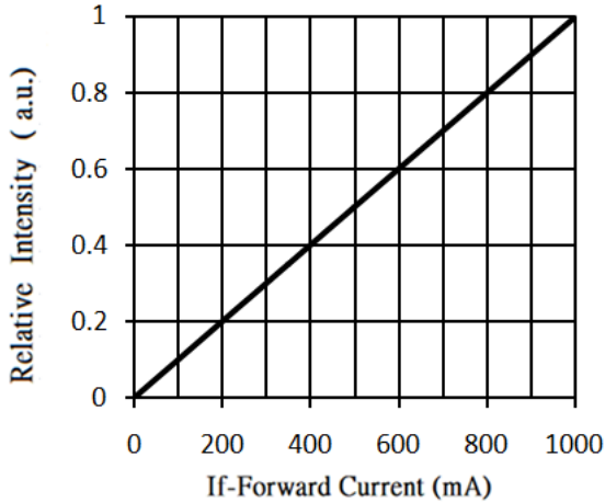
Fig.1-Relative Intensity VS. Forward Current
